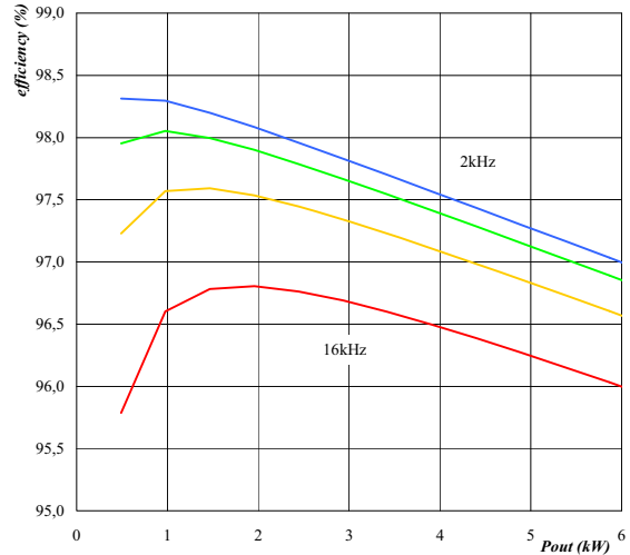
Figure 10. Typical efficiency as a function of output power Inverter \text{efficiency}=f(P_{out})
