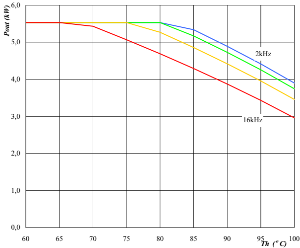
Figure 9. Typical available electric peak output power as a function of heatsink temperature Inverter P_{out}=f(T_h)
