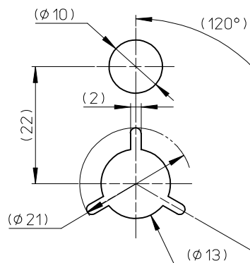
DETAIL "D"
