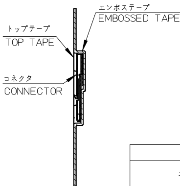
SECTION Y-Y
