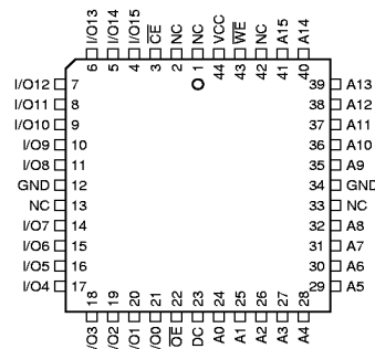
PLCC Top View
