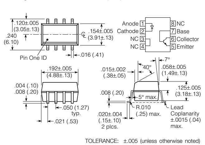
Package Dimensions in Inches (mm)
