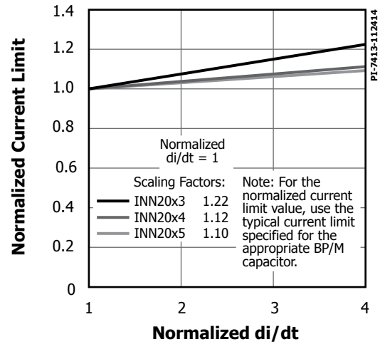
Figure 24. Standard Current Limit Vs. di/dt.
