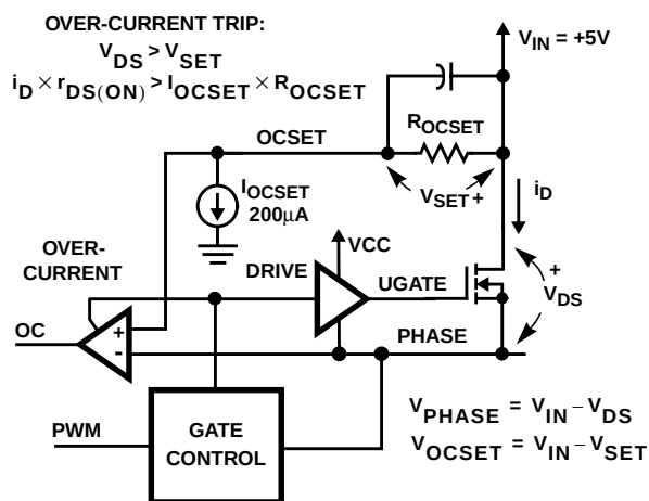
FIGURE 5. OVER-CURRENT DETECTION
