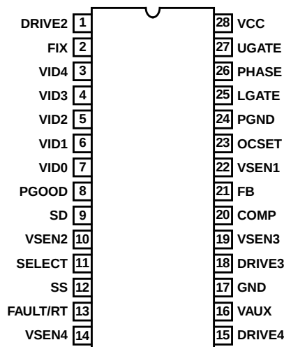
HIP6021A (SOIC) TOP VIEW
