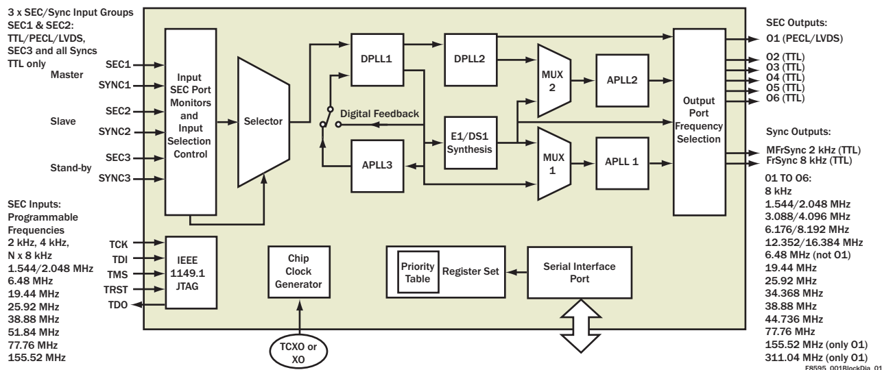
Figure 1 Block Diagram of the ACS8595 ATCA
