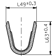
SECT. X-X
