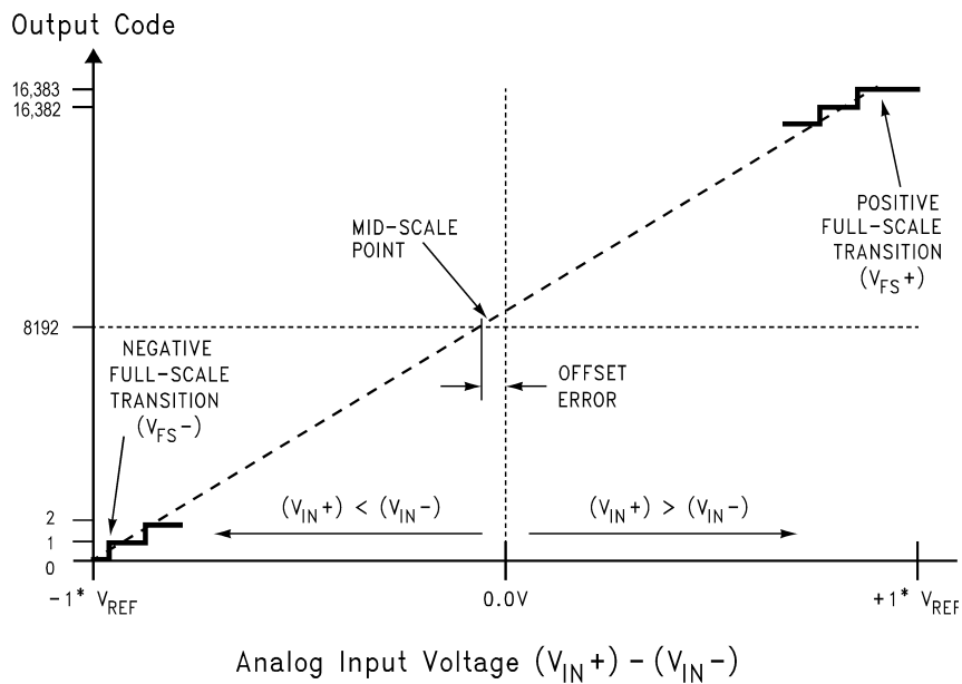
Figure 4. Transfer Characteristic
