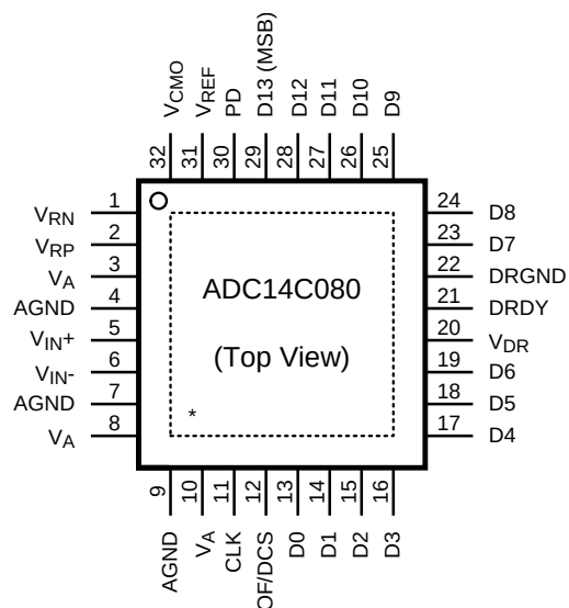
Figure 1. WQFN Package See Package Number RTV0032A
