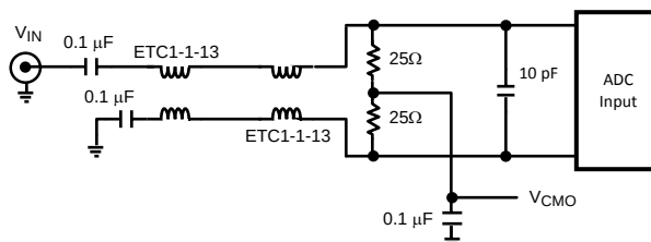
Figure 35. High Input Frequency Transformer Drive Circuit
