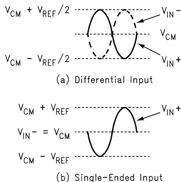
Figure 32. Expected Input Signal Range
