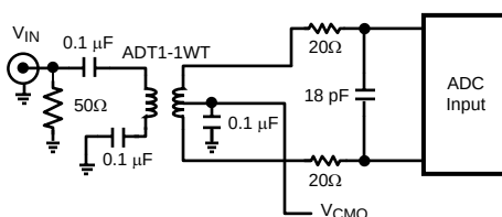
Figure 34. Low Input Frequency Transformer Drive Circuit
