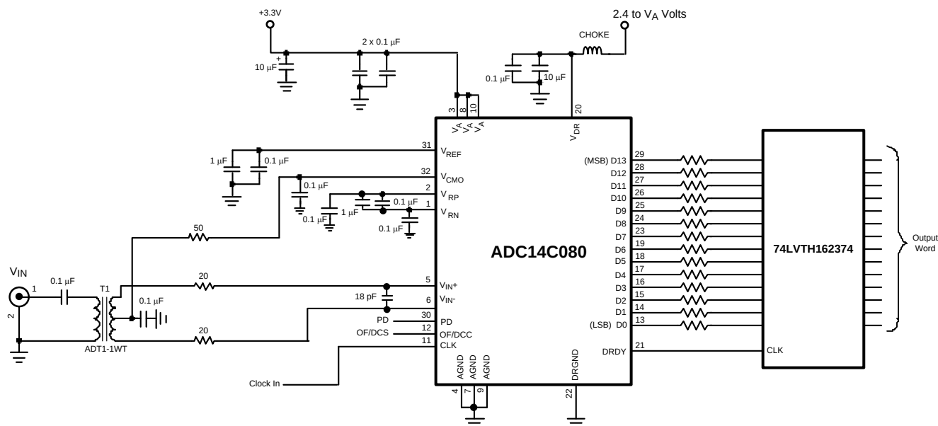
Figure 36. Application Circuit
