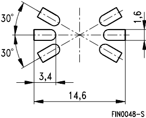
Recommended pad arrangement
