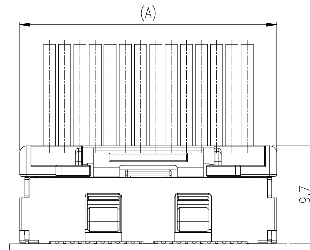
MATED CONNECTORS
