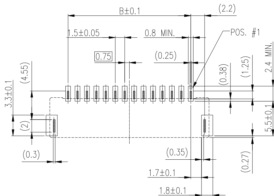
RECOMMENDED P.C.B. BOARD LAYOUT GENERAL TOLERANCE ±0.05
