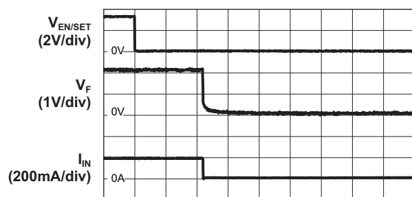
Turn-Off from 1.5x Mode Backlight
