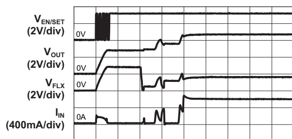
Turn-On to 2x Mode Flash
