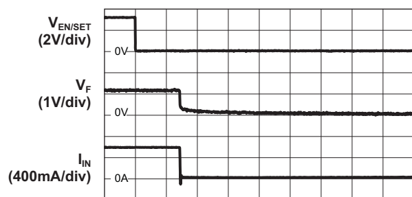
Turn-Off from 2x Mode Flash
