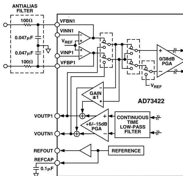
Figure 25. Analog Input (DC-Coupled)
