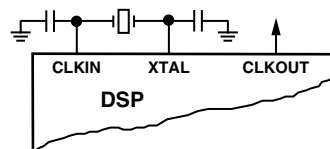
Figure 14. External Crystal Connections
