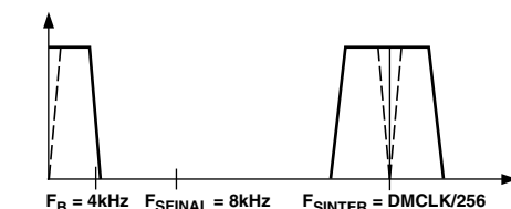
d. Final Filter LPF (HPF) Transfer Function Figure 5. ADC Frequency Responses
