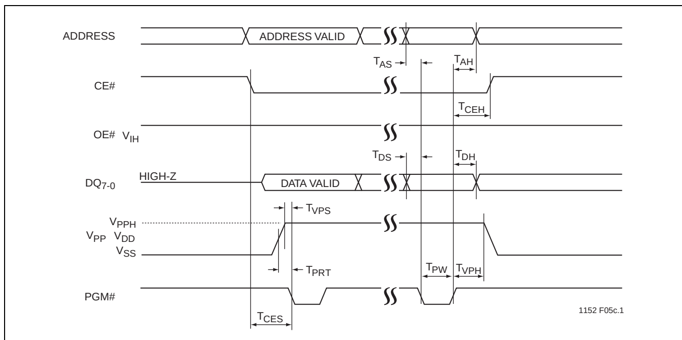
FIGURE 10: Byte-Program Timing Diagram for GLS27SF010/020
