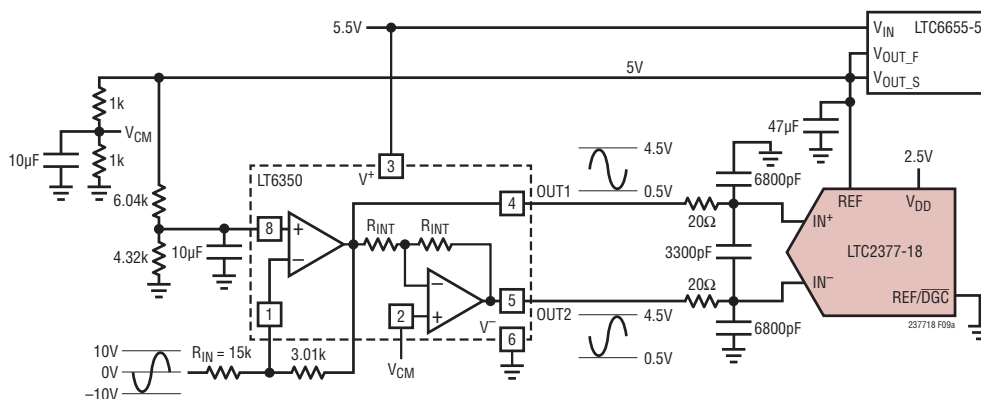
Figure 9a. LT6350 Configured to Accept a \pm 10\text{V} Input Signal While Running Off of a Single 5.5V Supply When Digital Gain Compression Is Enabled in the LTC2377-18
