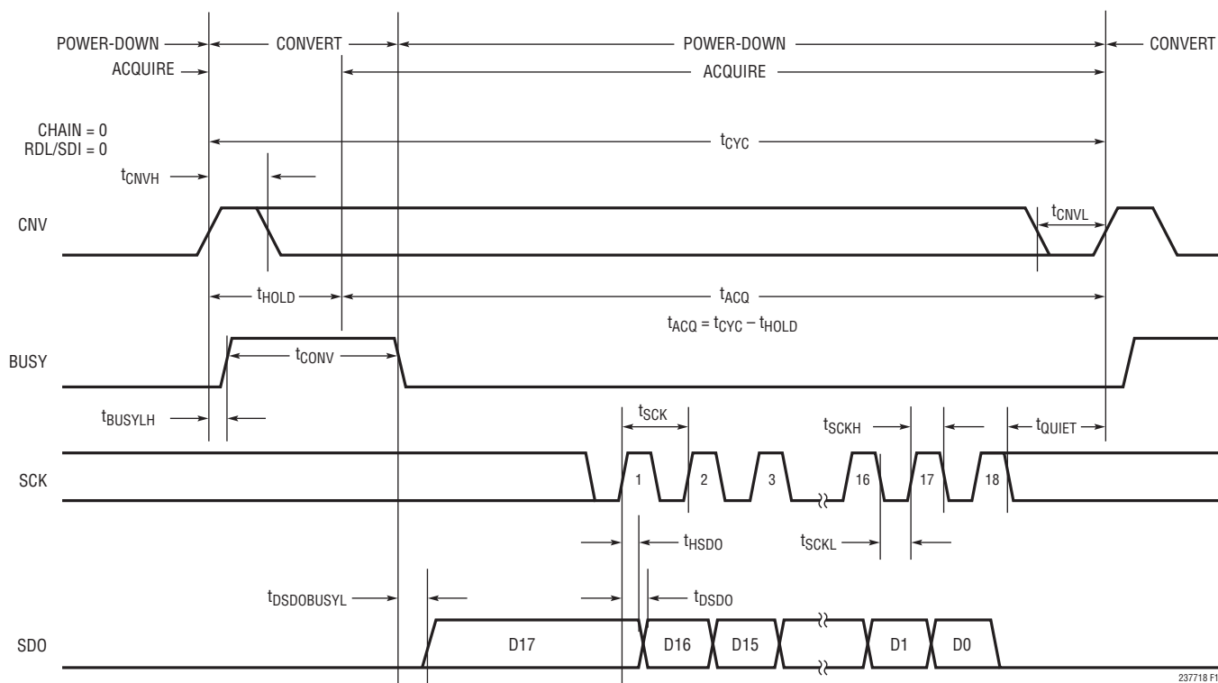
Figure 13. Using a Single LTC2377-18 in Normal Mode
