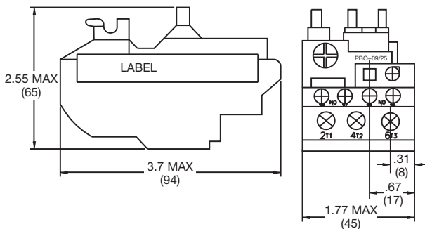
PBO-09, PBO-12, PBO-18 & PBO-25
