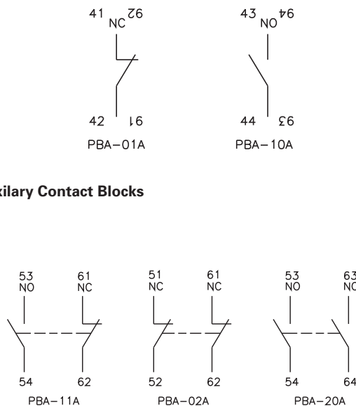
PBA-11A, PBA-02A & PBA-20A Front Mount Auxiliary Contact Blocks
