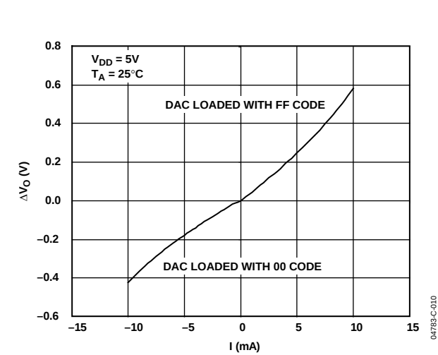
Figure 10. Source and Sink Current Capability
