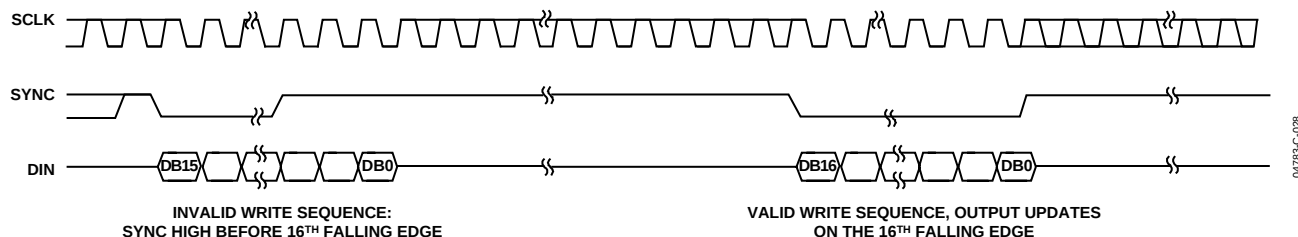
Figure 27. \overline{\text{SYNC}} Interrupt Facility
