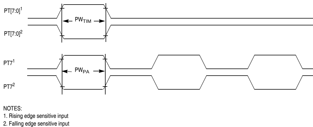
Figure 20-1. Timer Inputs
