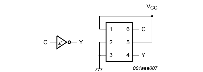
Figure 13. Inverter
