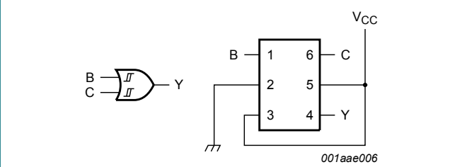
Figure 12. 2-input OR gate
