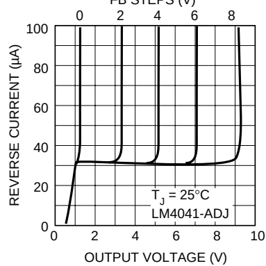
Reverse Characteristics †
