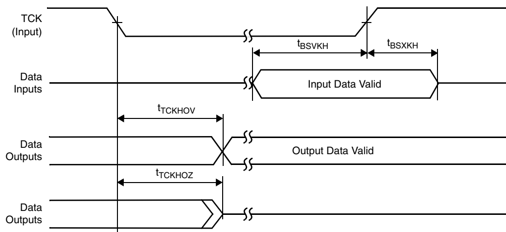
Figure 30. Boundary Scan (JTAG) Timing
