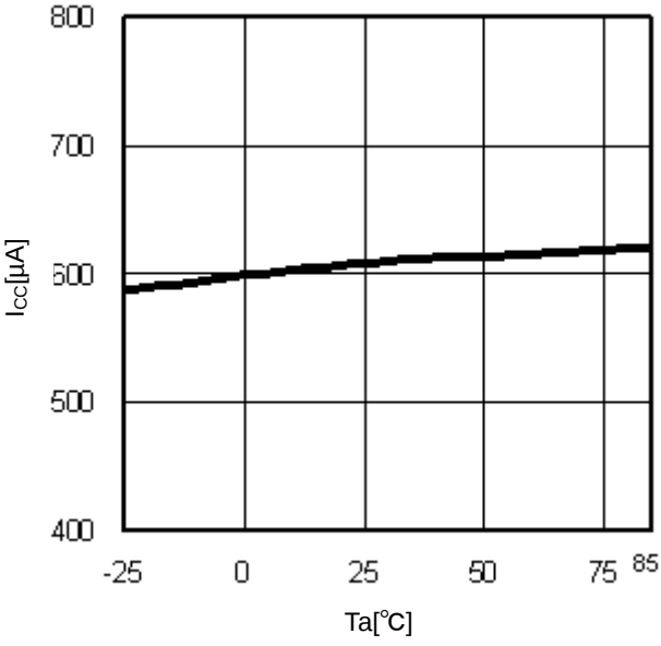
Figure 10. T_a-I_{cc}
