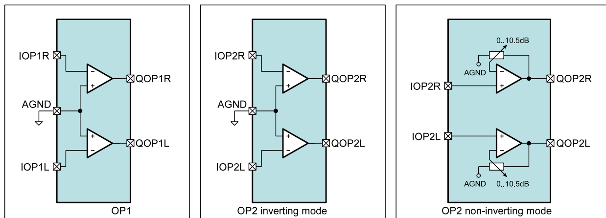
Figure 19. Operational Amplifiers
