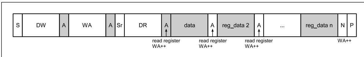
Figure 27. Sequential Read
