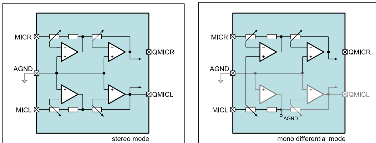
Figure 17. Microphone Input
