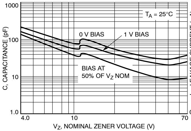
Figure 3. Typical Capacitance
