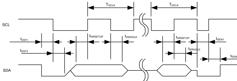
Figure 10 I 2 C Timing
