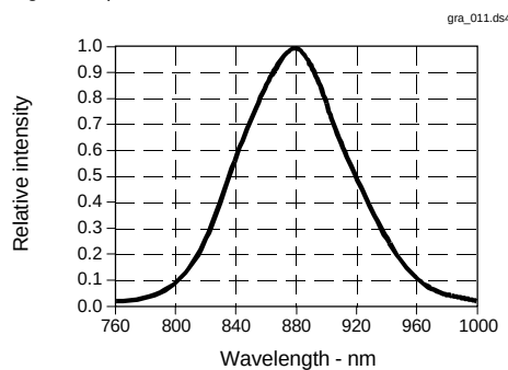
Fig. 5 Spectral Bandwidth
