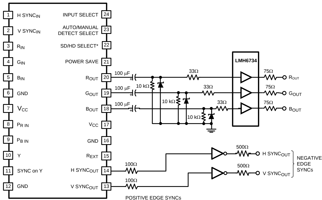
Figure 8. Simplified Application Diagram for Driving a VGA Cable
