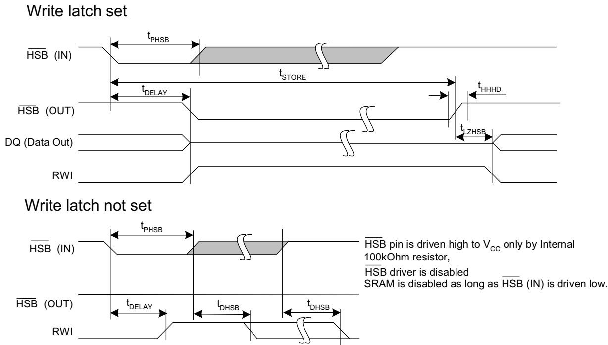
Figure 14. Hardware STORE Cycle [21]
