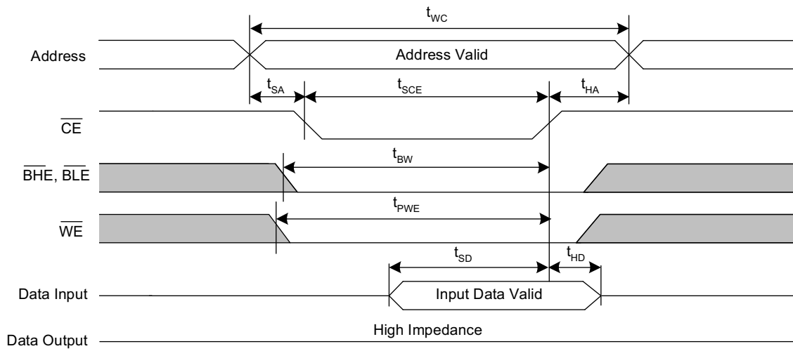
Figure 9. SRAM Write Cycle #2: \overline{\text{CE}} Controlled [3, 17, 18, 19]
