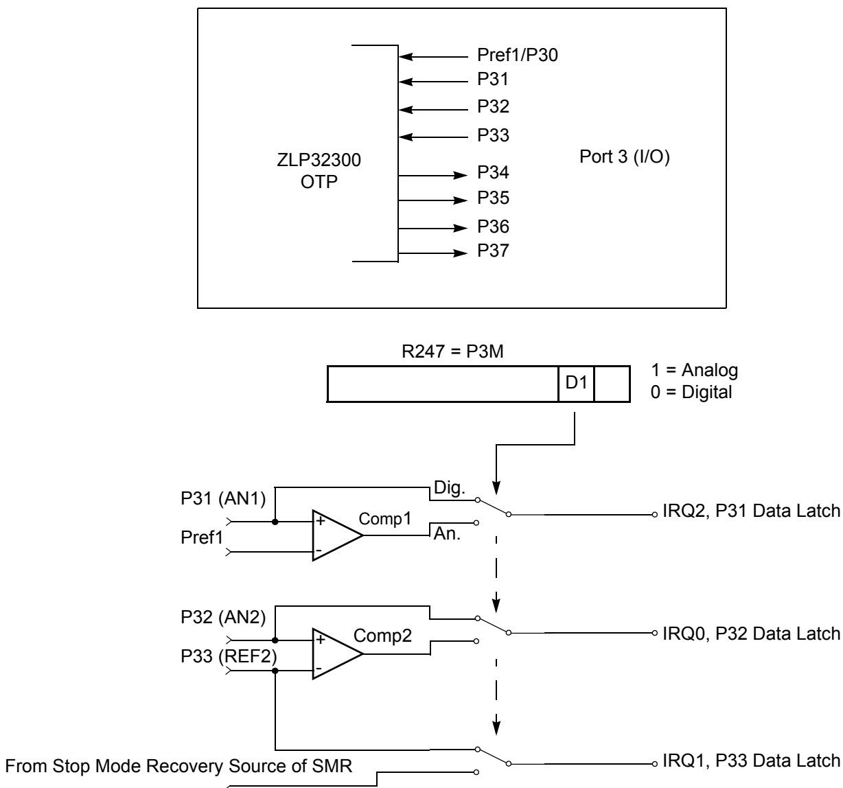
Figure 10. Port 3 Configuration
