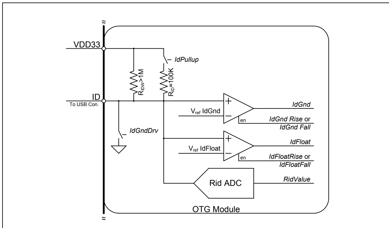
FIGURE 5-6: USB3340 ID RESISTOR DETECTION CIRCUITRY
