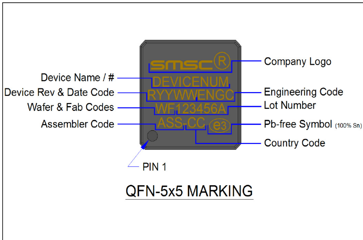
FIGURE 9-2: 32QFN, 5X5 PACKAGE MARKING
