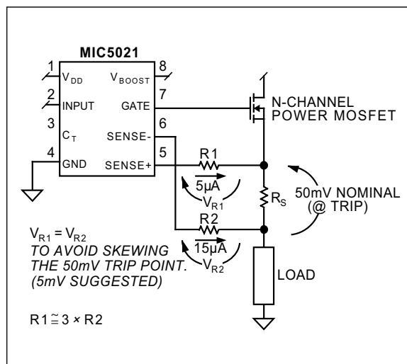
FIGURE 6-8: Resistor Voltage Drop.
