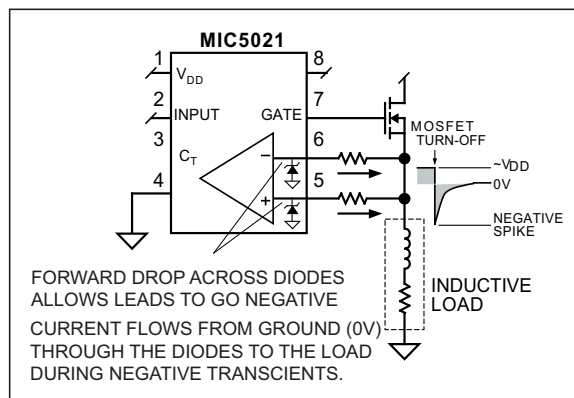
FIGURE 6-7: Inductive Load Turn-Off.
