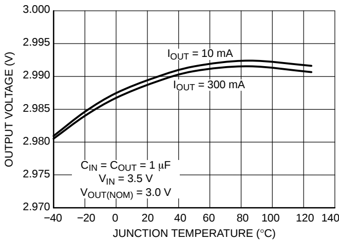
Figure 4. Output Voltage vs. Temperature V OUT = 3.0 V
