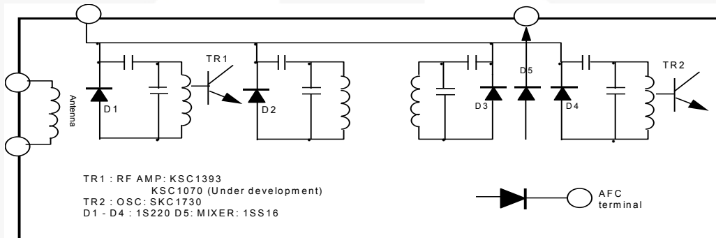
Figure 10. UHF Tuner
