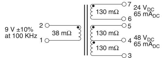
FLYBACK TRANSFORMER (approximately 10° C temperature rise)
