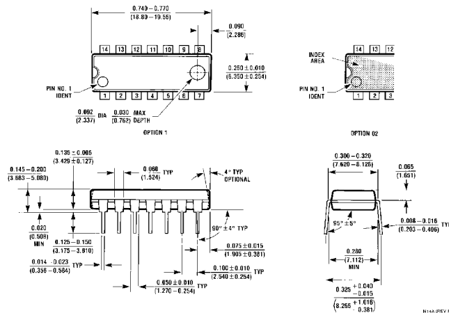
Molded Dual-In-Line Package (N) Order Number CD4024BMN or CD402BCN NS Package Number N14A
