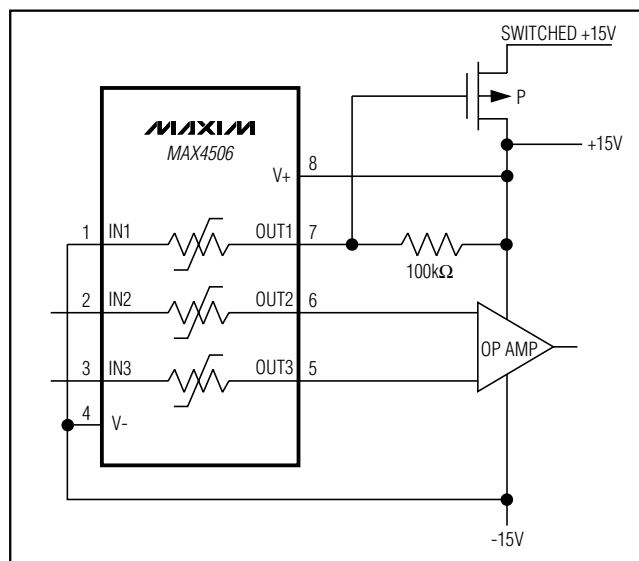
Figure 4. Power-Supply Sequencing
