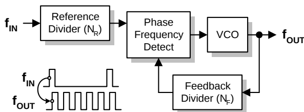
Figure 5: Simple PLL
