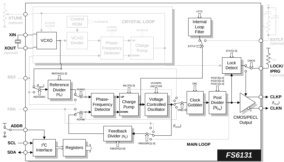
Figure 24: Block Diagram: Stand-Alone Clock Generation
