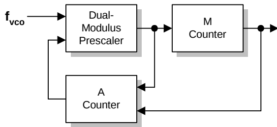
Figure 3: Feedback Divider
