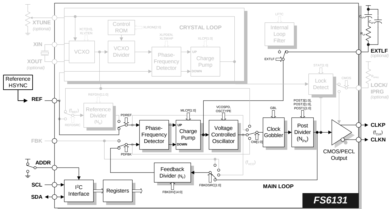
Figure 25: Block Diagram: Line-Locked Clock Generation
