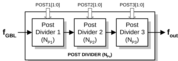
Figure 4: Post Divider
