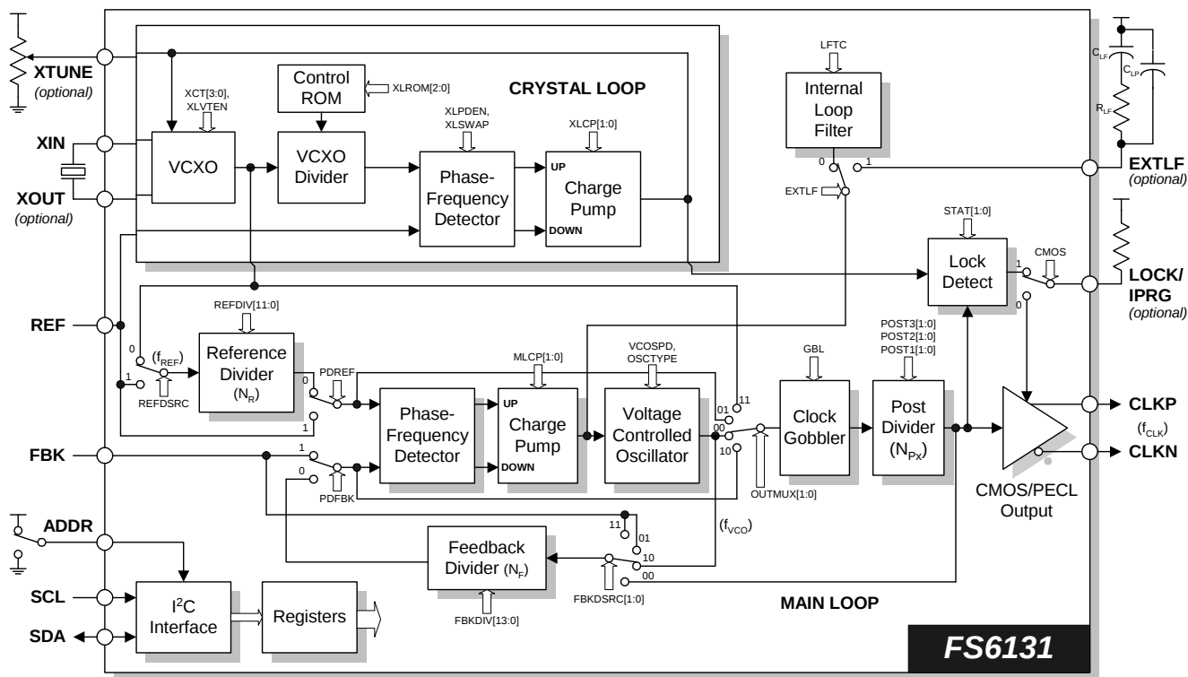
Figure 2: Block Diagram
