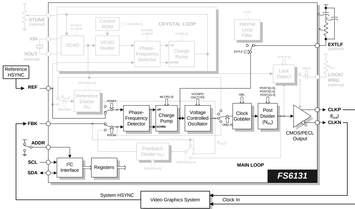
Figure 26: Block Diagram: Genlocking
