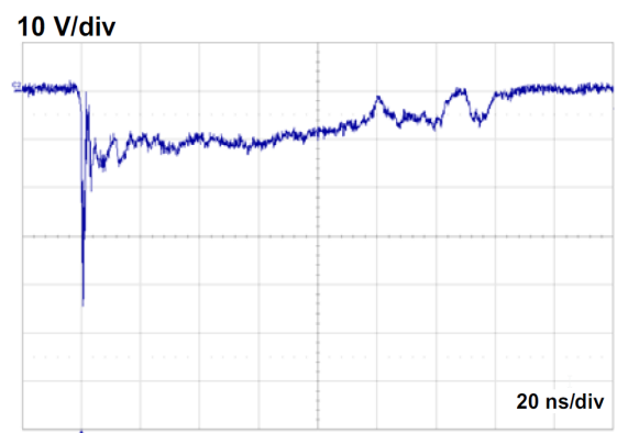
Figure 11. ESD response to ISO 10605, C = 150 pF, R = 330 \Omega (-8 kV contact)
