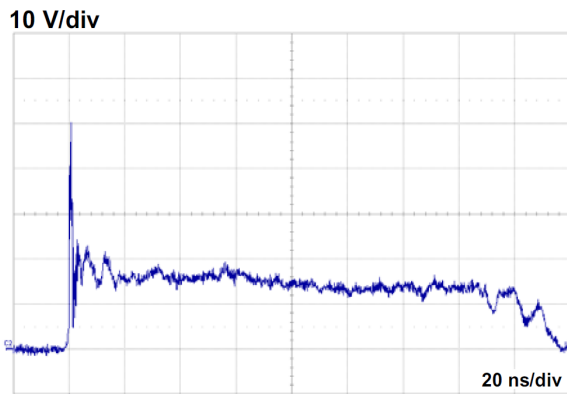
Figure 10. ESD response to ISO 10605, C = 150 pF, R = 330 \Omega (+8 kV contact)
