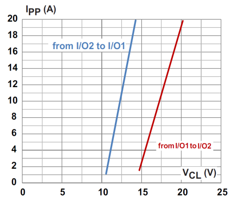
Figure 9. TLP measurements
