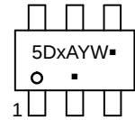
TSOP-6 (SOT23-6) SN SUFFIX CASE 318G STYLE 13
