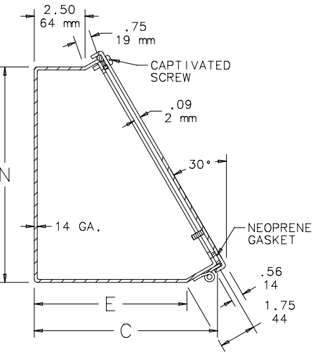
SECTION Y-Y
