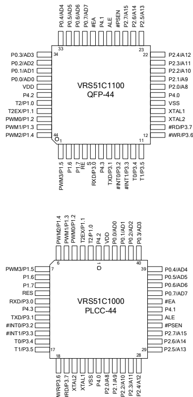
FIGURE 2: VRS51C1100 OFP-44 AND PLCC-44 PIN OUT DIAGRAMS
