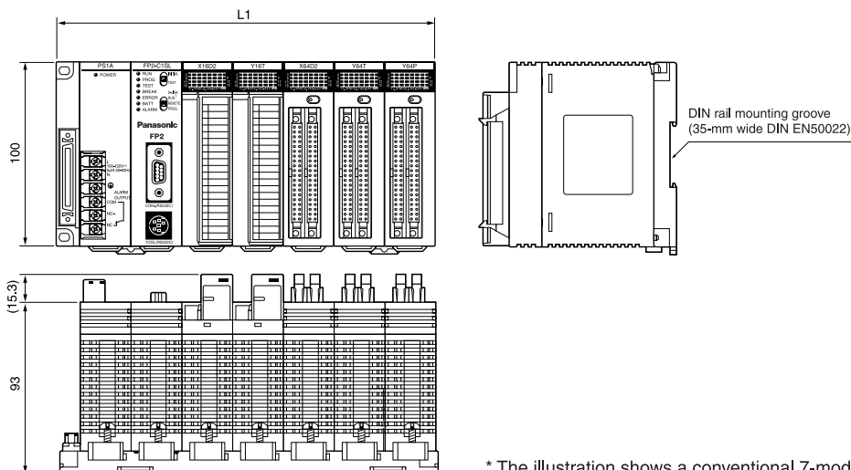
Mounting dimension (Tolerance: \pm 1.0 )
