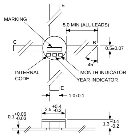
PACKAGE OUTLINE 07
