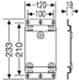
Dimension drawing
