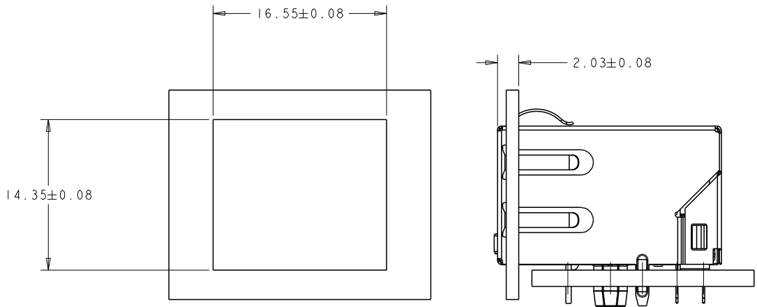
SUGGESTED PANEL CUTOUT SCALE 4:1
