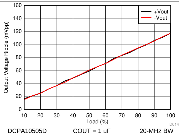
Figure 14. Output Ripple versus Load
