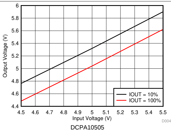
Figure 4. Line Regulation
