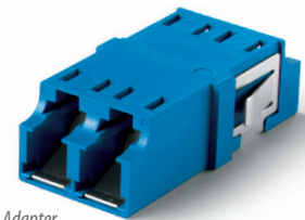
LC One Piece Adapter with SC Foot Print
