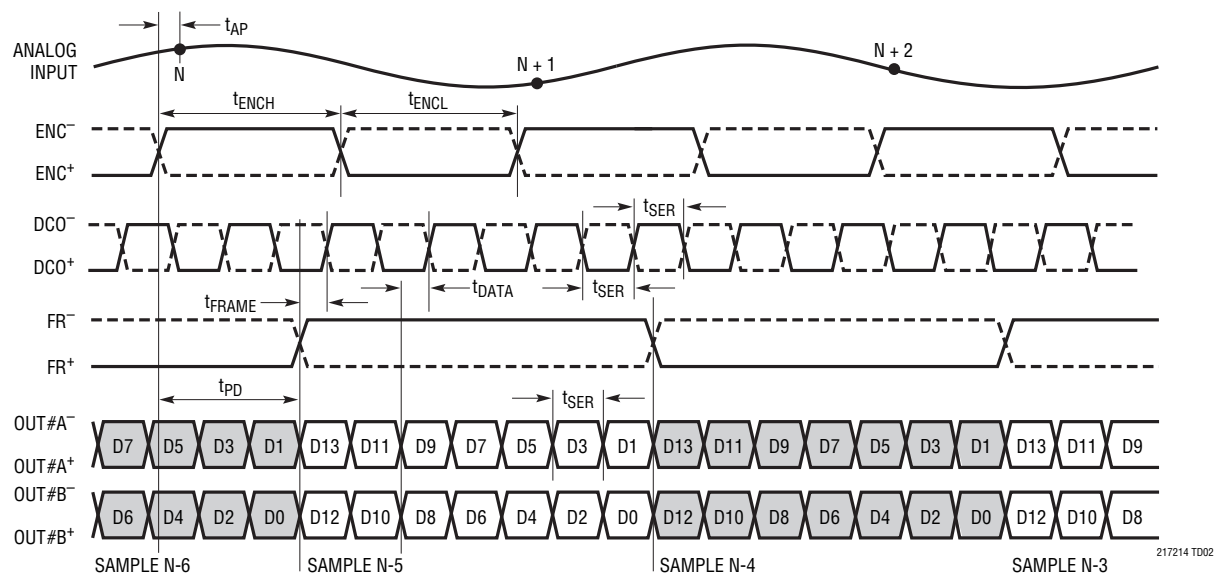
2-Lane Output Mode, 14-Bit Serialization
