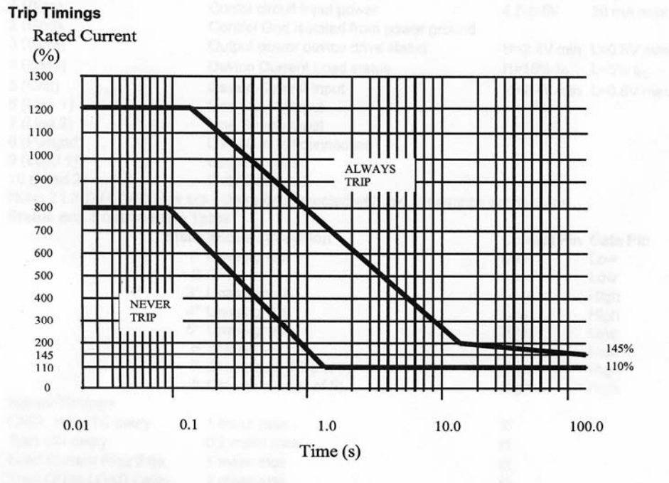
Figure 2 - Timing Diagram
