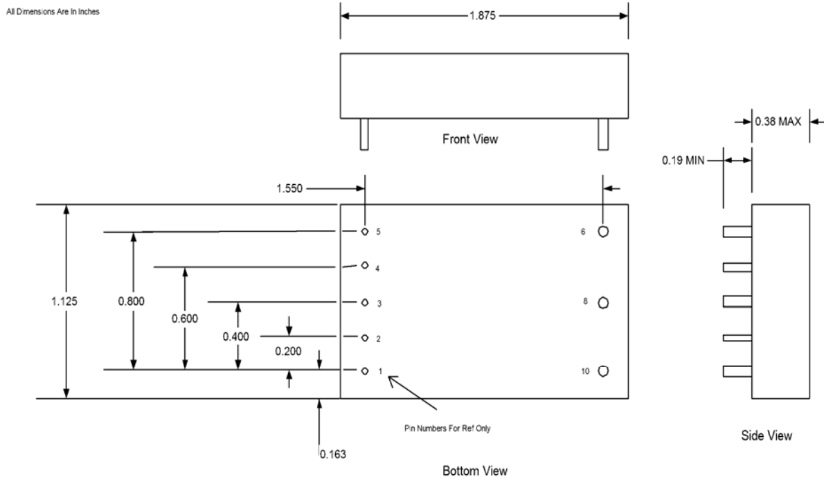
Figure 3 - Mechanical Dimensions
