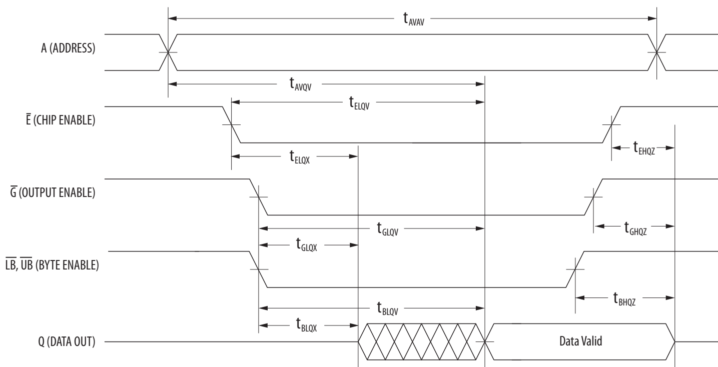
Figure 7 – Read Cycle 2
